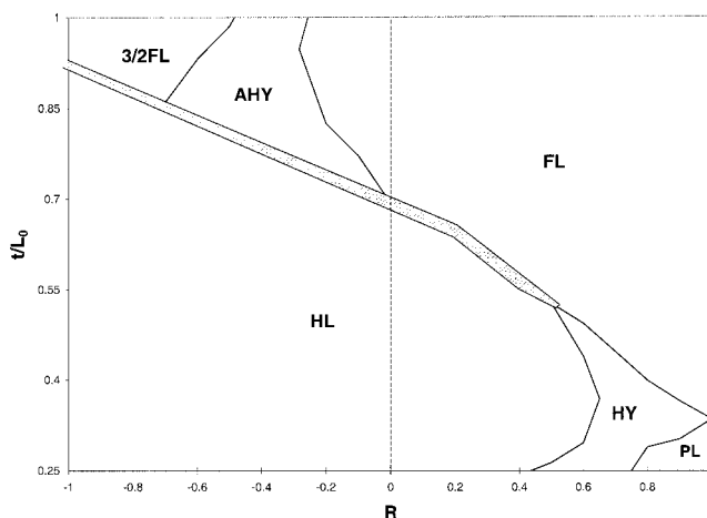
Figure 9. Complete (symmetric + antisymmetric) phase diagram for N = 150 , S_1^B = -0.3 kT, and \chi_{AB} = 0.1 . Phase fields are labeled with abbreviations from Figure 8. The gray area delineates where the HY structure is metastable.
